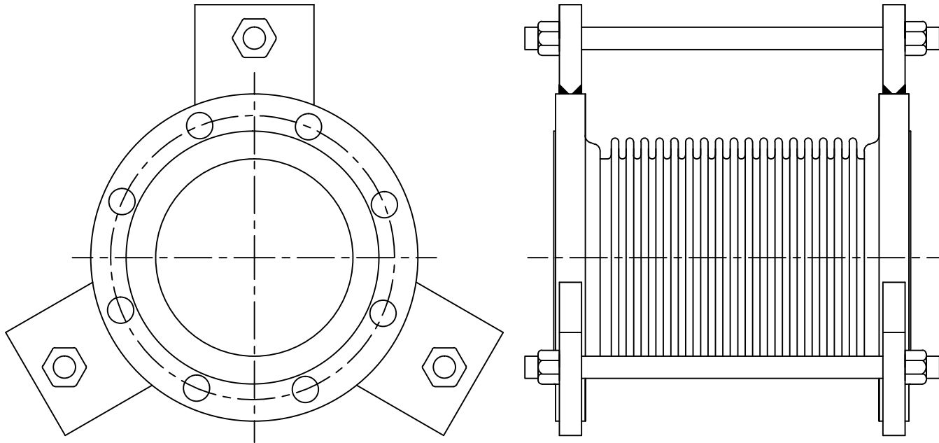
TITLE: SINGLE RESTRAINED FLANGED METAL BELLOW EXPANSION JOINT DESCRIPTION: DESIGNED FOR HIGHER PRESSURE, TEMPERATURE, AXIAL COMPRESSION , LATERAL OFFSET AND ANGULAR DEFLECTION
